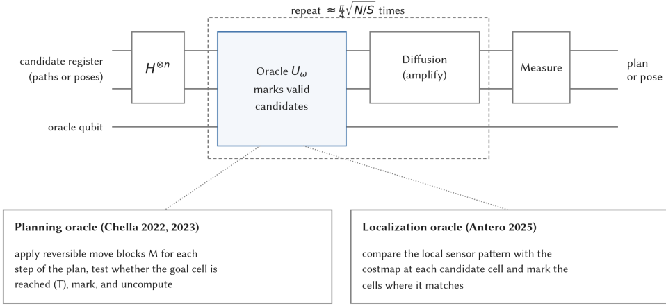
Fig. 5. Grover search as used for robot planning and localization. After a uniform superposition, the oracle marks goal-reaching action sequences [28, 29] or map cells whose stored pattern matches the current sensor view [4], and the diffusion step amplifies the marked states; about \frac{\pi}{4} \sqrt{N/S} repetitions are needed for N candidates and S solutions. Redrawn from the circuit descriptions in those studies.
