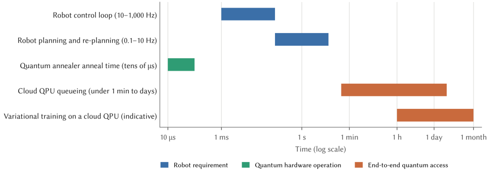
Fig. 10. Timescales of robot control and planning compared with quantum hardware operation and end-to-end cloud quantum access (log scale). The anneal time is from Ohzeki et al. [122] and the queueing range from Ravi et al. [138]; the range for variational training is indicative.
