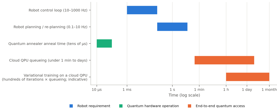
Fig. 6. Timescales of robot control and planning compared with quantum hardware operation and end-to-end cloud quantum access (log scale). The anneal time is from Ohzeki et al. [104] and the queueing range from Ravi et al. [117]; the range for variational training is indicative.
