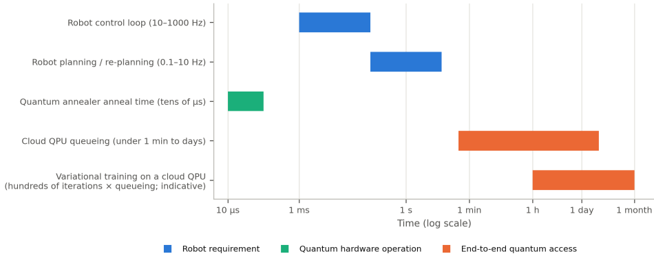
Fig. 5. Timescales of robot control and planning compared with quantum hardware operation and end-to-end cloud quantum access (log scale). The anneal time is from Ohzeki et al. [104] and the queueing range from Ravi et al. [117]; the range for variational training is indicative.
