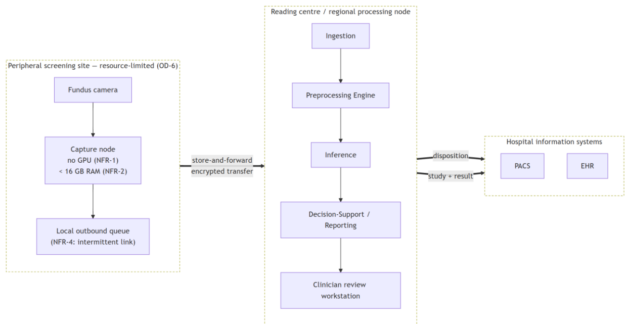
Diagram C.2 – Store-and-forward deployment topology (DIA-6.3b)
