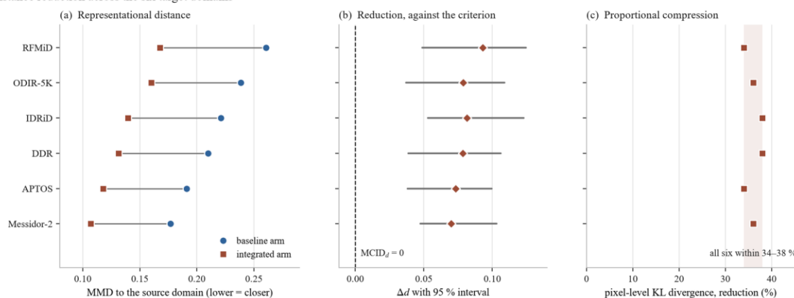
Domain-distance reduction across the six target domains
