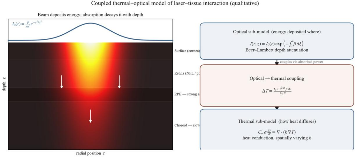
Figure 2.3 – Coupled thermal-optical model of laser-tissue interaction – Gaussian-beam intensity, Beer–Lambert depth attenuation, and heat conduction across fundus layers
