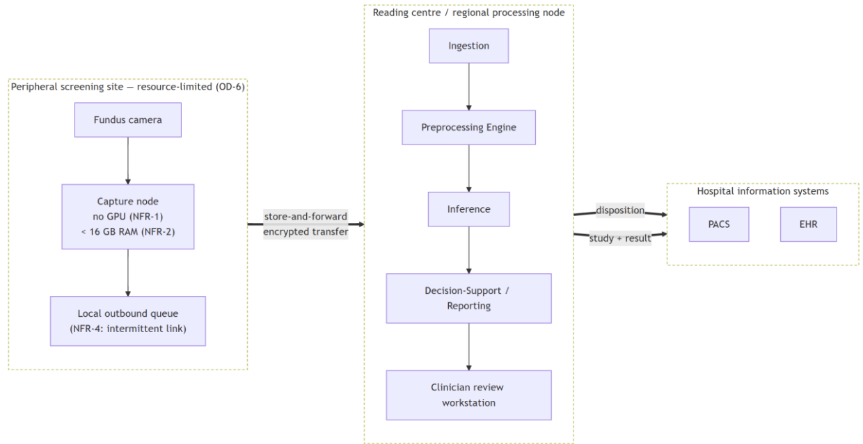
Diagram C.2 – Store-and-forward deployment topology
