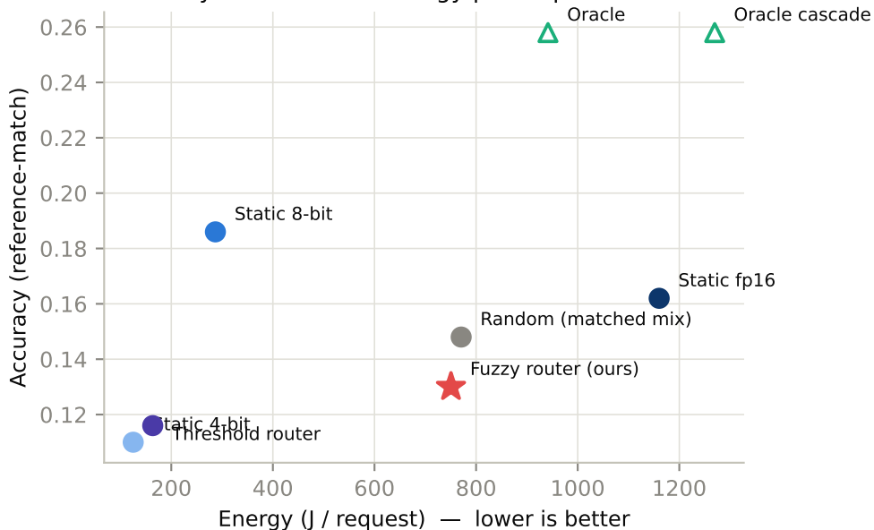
Accuracy vs measured energy per request
