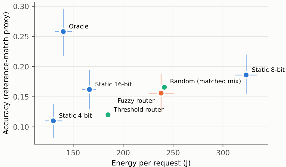
Routing conditions, run 5 (95% bootstrap CIs)
