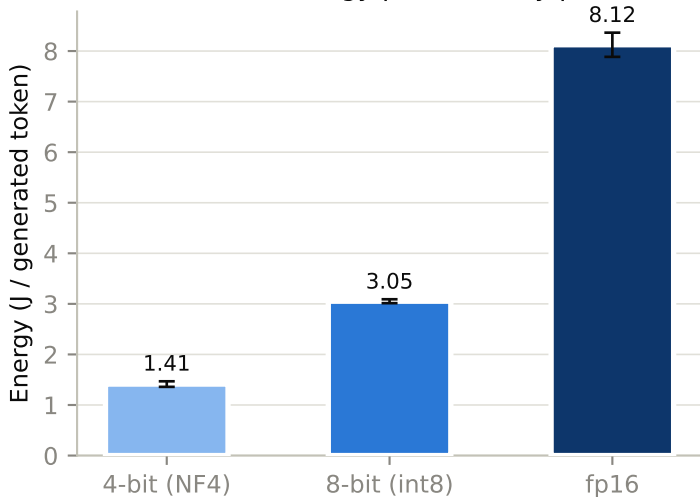
Measured GPU energy per token by precision tier
