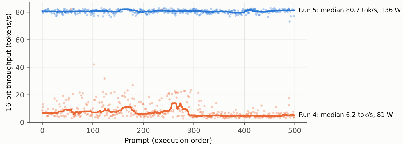
Same model, same GPU: 16-bit throughput in a disrupted vs. clean run
