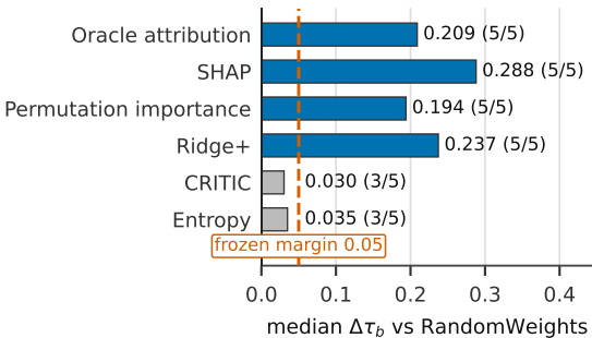
A Structured information vs RandomWeights
