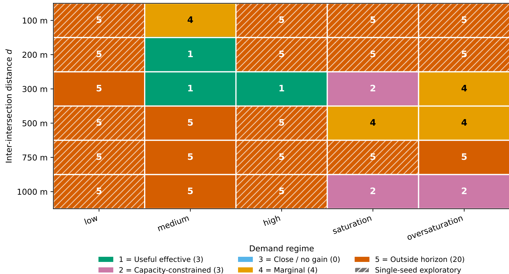
Integrated DCHF diagnosis: distance \times demand
