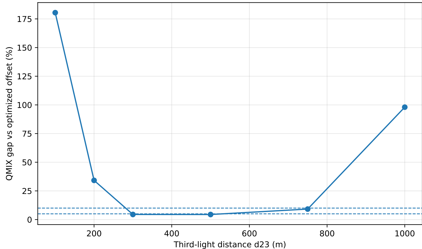
Three-intersection third-light horizon: QMIX approximation gap
