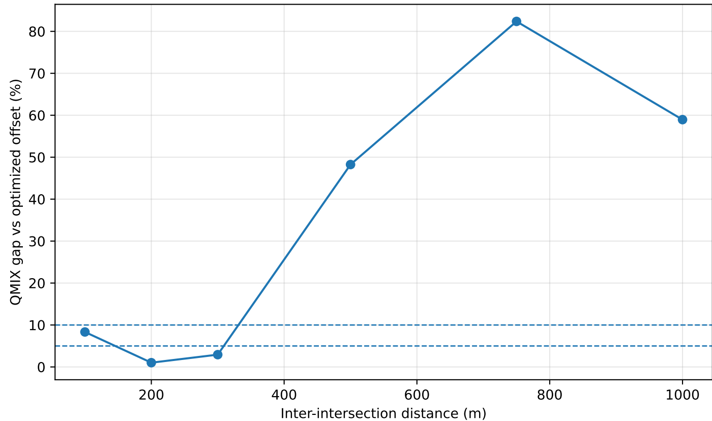
Two-intersection spatial horizon: QMIX approximation gap
