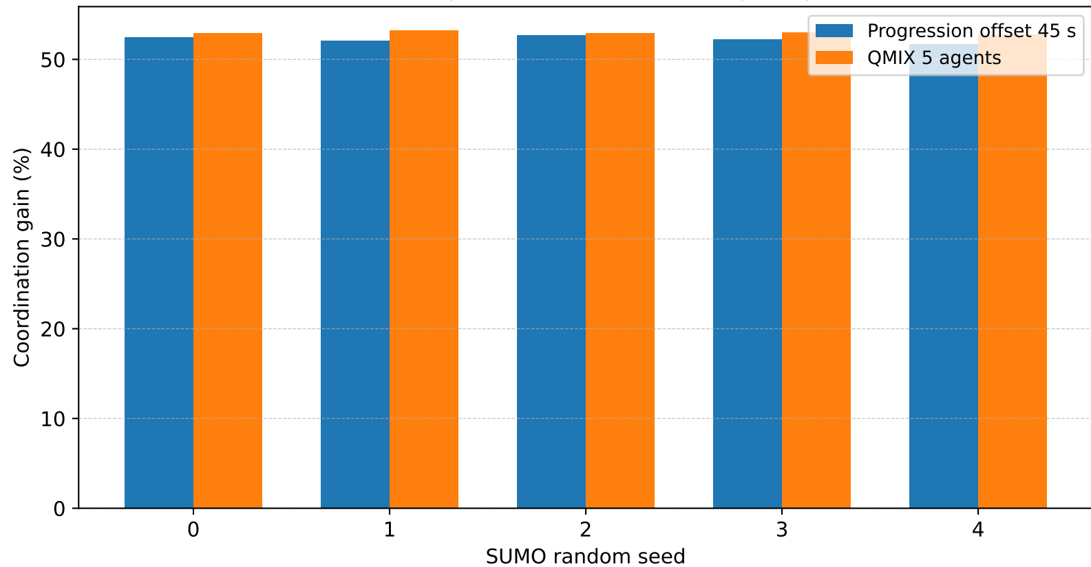
N=5 scalability validation: coordination gain by seed
