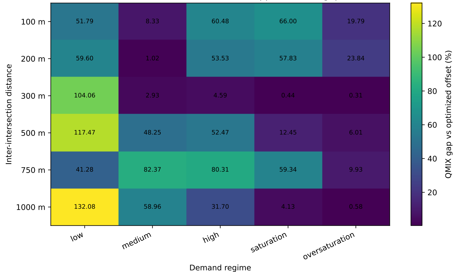
Distance \times Demand DCHF: QMIX approximation gap
