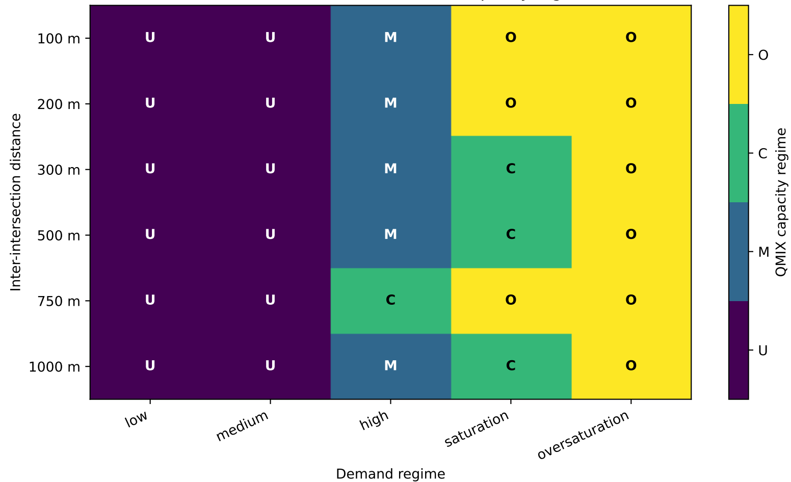
Distance × Demand DCHF: QMIX capacity regime
