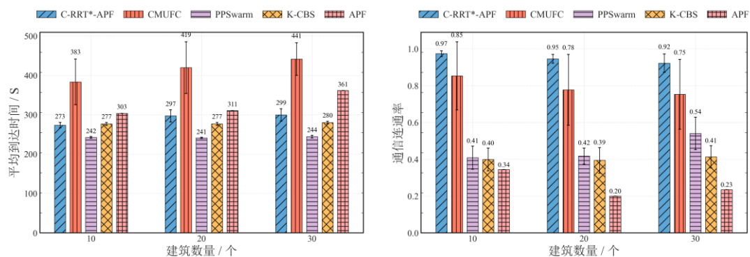
(a) Comparison of average arrival time under different building numbers (b) Comparison of communication connectivity rate under different building numbers
