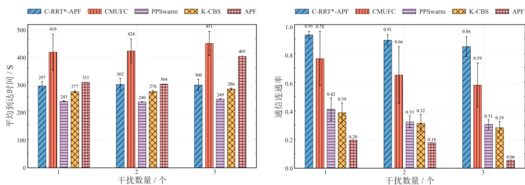
(e) Comparison of average arrival time under different numbers of interference (f) Comparison of communication connectivity rate under different numbers of interference
