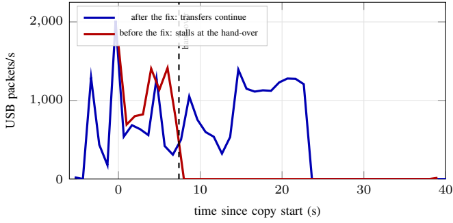
Fig. 6. USB packets per second across the hand-over, counted by usbmon at the vfio-user server. Both traces are single runs, so this is an illustration of the mechanism rather than a controlled A/B comparison. Without the interrupt fix the transfers stop at the hand-over and do not recover within the observed window; with the fix they continue until the copy completes.
