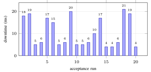
Fig. 4. Measured downtime of the 20 acceptance runs (source: data/runs.dat, from results-debug.csv). The goal of \leq 2000 ms is far above the plotted range.
