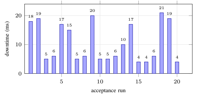
Fig. 4. Measured downtime of the 20 acceptance runs. The goal of \leq 2000 ms is far above the plotted range.
