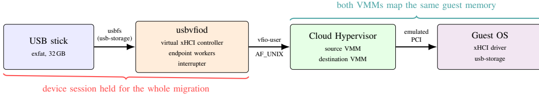
Fig. 1. System architecture. usbvfiod owns the physical USB device and emulates an xHCI controller; the VMM reaches it over vfiio-user. During a same-host migration the server process is never restarted, so the device session and the controller state survive, and both VMMs map the same guest memory.
