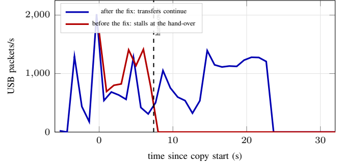
Fig. 6. USB transaction rate across the hand-over, measured at the vfiio-user server. Without the interrupt fix, transfers stop at the hand-over and never resume; with the fix they continue until the copy completes.
