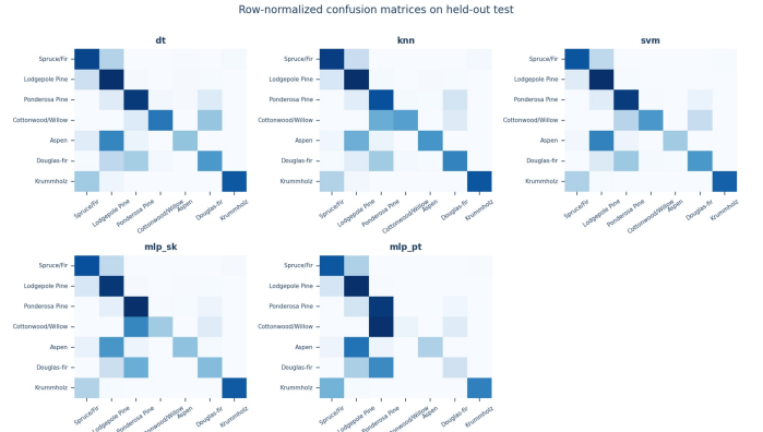
Fig. 4: Row-normalised confusion matrices. Diagonal mass = per-class recall; off-diagonal mass shows the dominant confusions.
