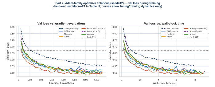
Fig. 2: Part 2 — validation loss vs. GEs (left) and wall-clock time (right), all seven variants, seed= 42. The dotted line marks \ell_{\text{vis}}=0.671 , plotted as 90% of Adam’s initial validation loss — a visual reference showing where all methods have meaningfully departed from their starting point. This is distinct from the \ell=0.539 threshold (90% of SGD-no-mom’s initial loss) used in Table III’s GEs-to- \ell column for speed comparisons. Adam-family methods cross \ell_{\text{vis}} within the first 50–100 GEs; SGD-no-momentum does not cross it until \approx 1,300 GEs, confirming H1. The Adam (no bias-correction) curve sits above standard Adam for the first 10 epochs then converges to the same basin, confirming that bias correction primarily matters early [8]. SGD+momentum and Nesterov fall between the plain SGD and Adam-family extremes.
