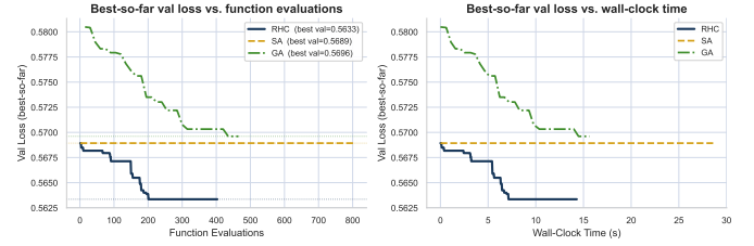
Fig. 1: Part 1 — best-so-far validation loss vs. function evaluations (left) and wall-clock time (right) for RHC, SA, and GA. RHC (solid) descends steeply in the first 200 FEs then plateaus at the local optimum it cannot escape without restarts; SA (dashed flat) begins at its best value (0.5689) and never improves — with T_0=1.0 , T_{\text{decay}}=0.995 , and \Delta\theta \sim \mathcal{N}(0, 0.01^2) , the temperature collapses within \sim 150 steps and all Metropolis proposals are rejected, freezing the chain at the initial point; GA (dotted) descends gradually across generations but burns \approx 3\times the FEs of RHC for inferior final loss. SA’s failure to explore is itself a result: it shows that geometric cooling at this rate is too aggressive for the 1,159-parameter landscape after gradient descent has already found a well-conditioned basin. This is the RO-limited-gains signature H3 predicts.
