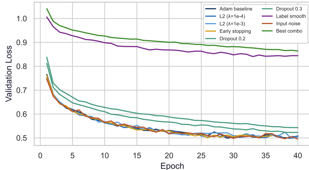
Val loss vs. epoch (seed=42)
