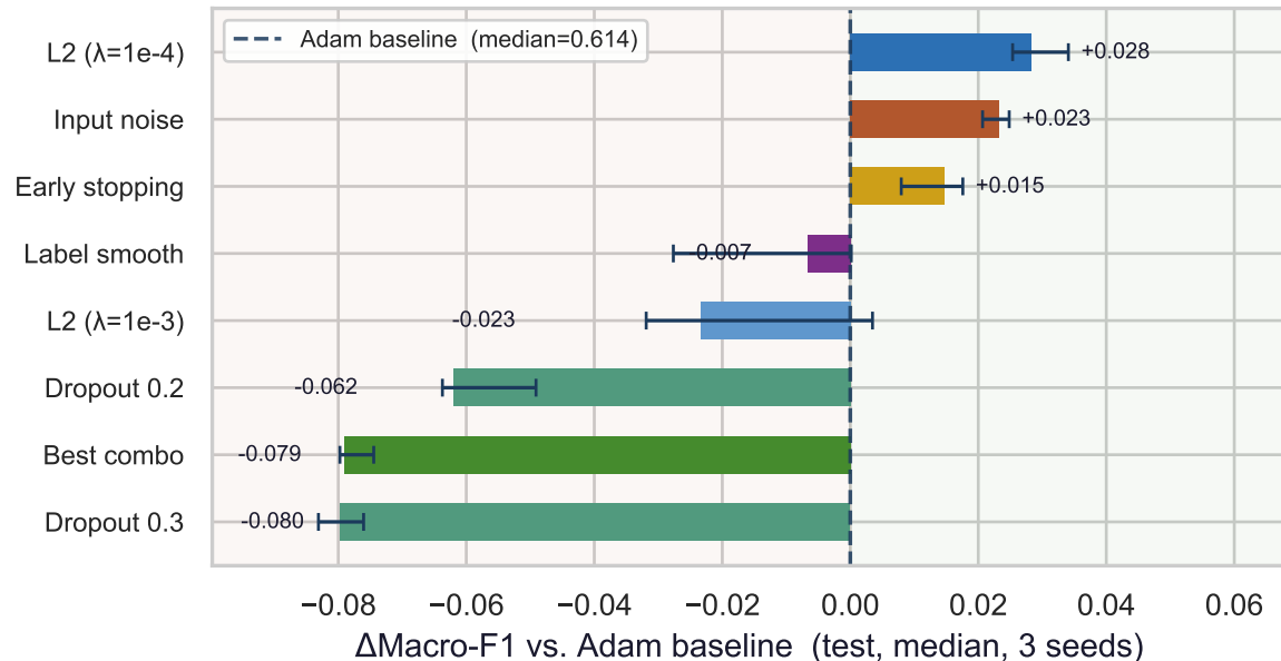
Macro-F1 gain / loss vs. Adam baseline
