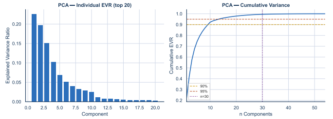
Fig. 4: Left: individual EVR for top-20 PCs — components 1–2 dominate, components beyond 14 contribute < 1\% each. Right: cumulative EVR with 90 % (amber dashed) and 95 % (sienna dashed) thresholds. n=30 (plum dotted) captures 99.5 %, providing a generous but stable embedding.
