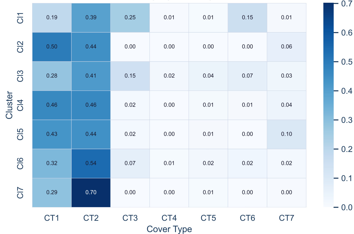
K-Means (k=7) × Cover Type
