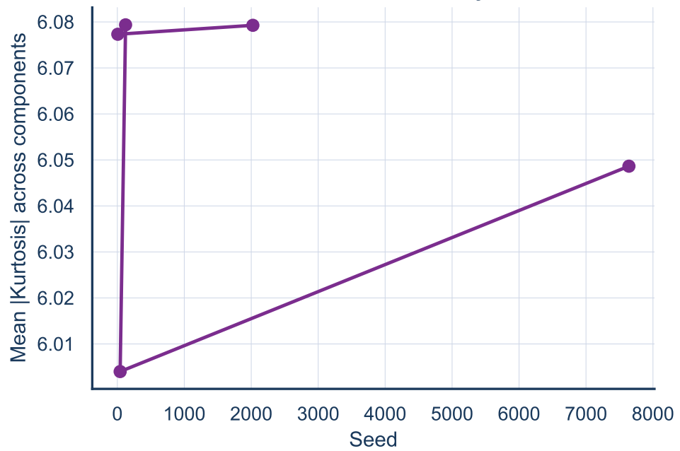
ICA — Seed Sensitivity
