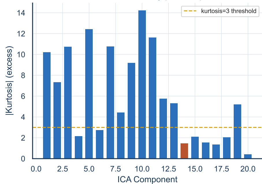
ICA — Non-Gaussianity per Component
