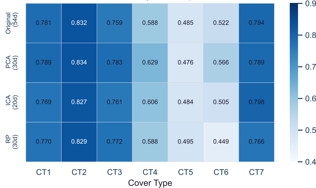
Per-class F1 by Feature Space
