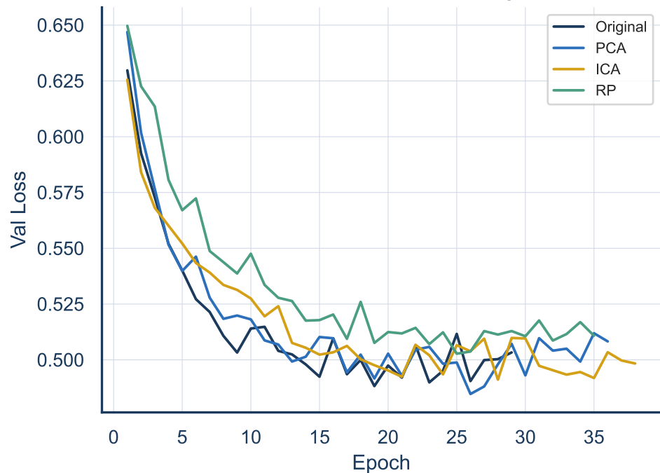
Validation Loss — All Feature Spaces
