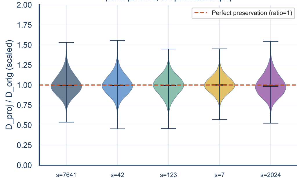
RP — Per-pair Distance Ratio Distribution (violin per seed, 500-point subsample)
