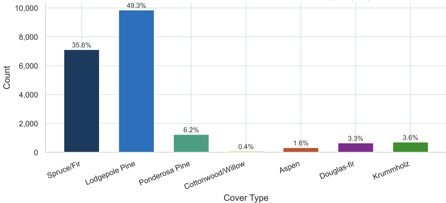
Class distribution — stratified 20k subsample (OL)
