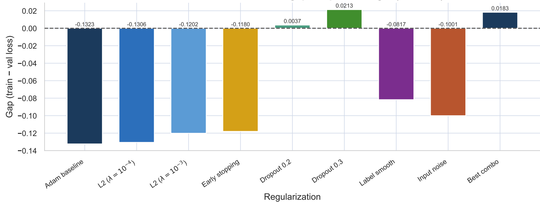
Part 3: Train – validation loss gap at epoch budget (seed=42)
