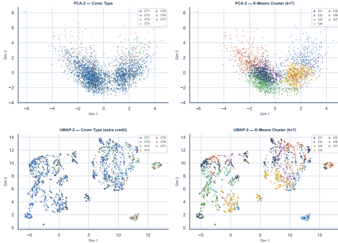
Fig. 9: 2D projections of the 20k Covertype sample (3,000-point subsample). Top row : PCA-2, coloured by Cover Type ( left ) and K-Means cluster ( right ). CT1/CT2 form overlapping clouds; PCA captures elevation variance but not ecological labels. Bottom row : UMAP-2 (extra credit; n_{\text{neighbors}}=30 , \text{min\_dist}=0.1 , seed 7641). Minority classes CT4, CT5, CT7 form tight isolated islands in UMAP space that are invisible in PCA-2. K-Means cluster assignments ( bottom right ) cut across these UMAP islands, showing elevation-driven clusters do not align with the non-linear manifold topology UMAP exposes.
