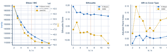
Fig. 2: Left : inertia and BIC sweeps — no sharp elbow at k=7 . Center : silhouette is highest at k=2 for K-Means; GMM silhouette is consistently lower, indicating its elliptical components do not match distance-based silhouette geometry. Right : ARI vs. Cover Type labels is low across all k , peaking at k=3 for GMM (ARI = 0.119), consistent with the two dominant classes (CT1, CT2) and an elevation-driven third grouping. Vertical dotted line = k=7 (reference).
