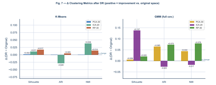
Fig. 7: \Delta clustering metrics after DR vs. original-space baseline (positive = improvement). Left (K-Means) : all three DR methods improve silhouette and NMI slightly; ICA hurts ARI (-0.028) because independent components disrupt the elevation-driven Euclidean structure K-Means relies on. Right (GMM) : ICA delivers the largest silhouette gain (+0.137) because whitening regularises full-covariance estimation; PCA dominates on ARI (+0.065) and NMI (+0.044); RP improves NMI (+0.078) but hurts ARI (-0.025) by destroying dominant-variance geometry. The asymmetry between K-Means and GMM responses directly tests H3.
