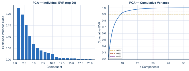
Fig. 4: Left : individual EVR for top-20 PCs — components 1–2 dominate, components beyond 14 contribute < 1\% each. Right : cumulative EVR with 90 % (amber dashed) and 95 % (sienna dashed) thresholds. n=30 (plum dotted) captures 99.5 %, providing a generous but stable embedding.
