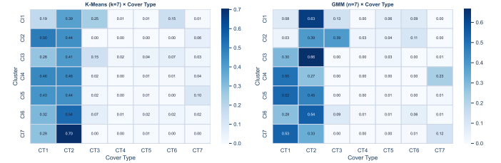
Fig. 3: Cluster \times Cover Type contingency (row-normalised) for K-Means ( left ) and GMM ( right ) at n=7 . K-Means clusters are dominated by CT1/CT2 with minority types spread thinly; GMM distributes more across clusters but still fails to isolate CT4 (rarest class).
