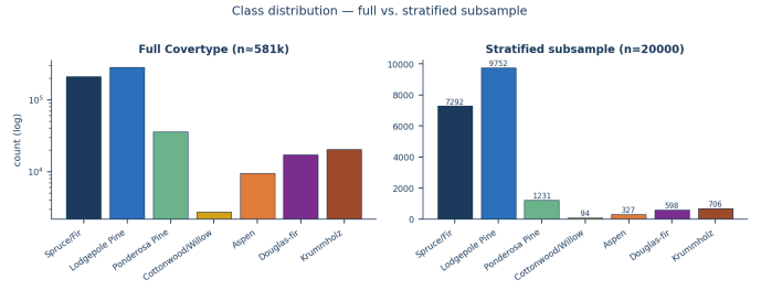
Fig. 1: Class distribution. Left : full Covertypes ( n \approx 581k , log-scaled). Right : stratified 20k subsample. Stratification preserves the long tail (Cottonwood/Willow \sim 0.47\% ) so per-class metrics are not degenerate.
