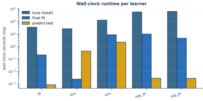
Fig. 5: Wall-clock seconds per learner (log-scaled): tuning total, final fit on 16k, and prediction on the 4,000-row test set.
