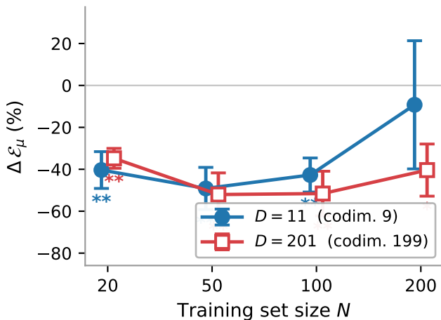
Paraboloid
