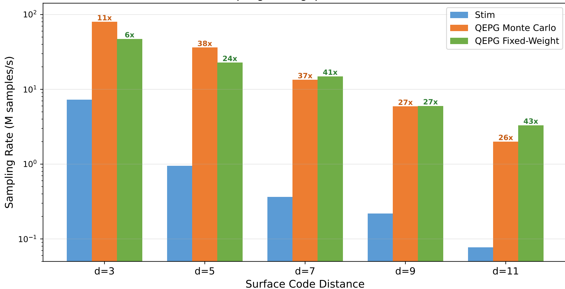
Detector Sampling Throughput: ScaLERQEC vs Stim
