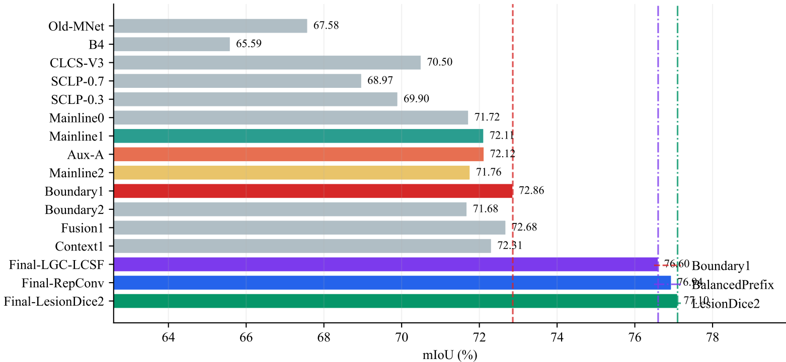
ATLSDS Training Results: mIoU Comparison
