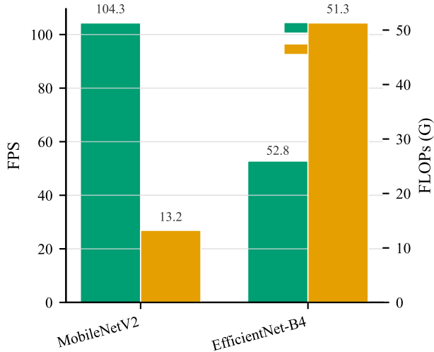
Inference cost
