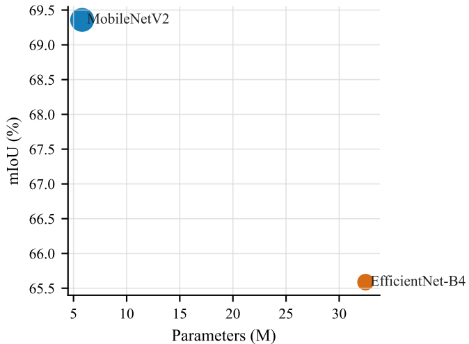
Accuracy-efficiency trade-off
