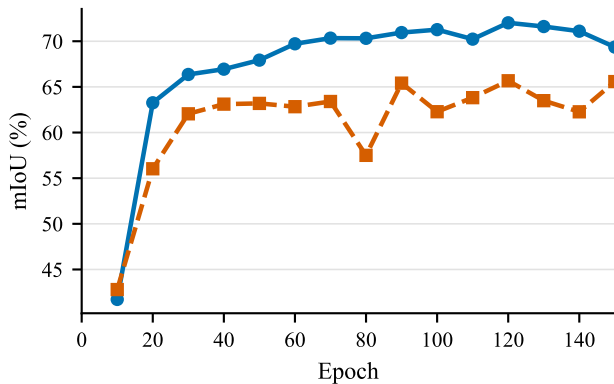
Validation mIoU
