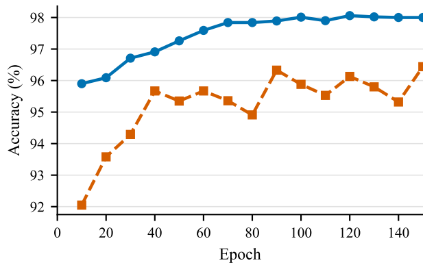
Pixel accuracy
