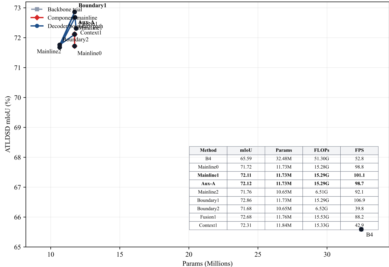
ATLSD Model Accuracy-Efficiency Comparison
