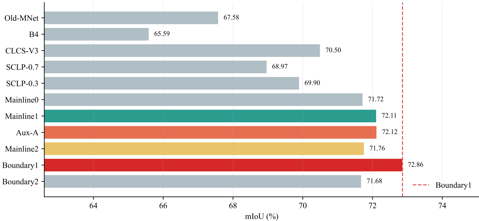
ATLDS Training Results: mIoU Comparison
