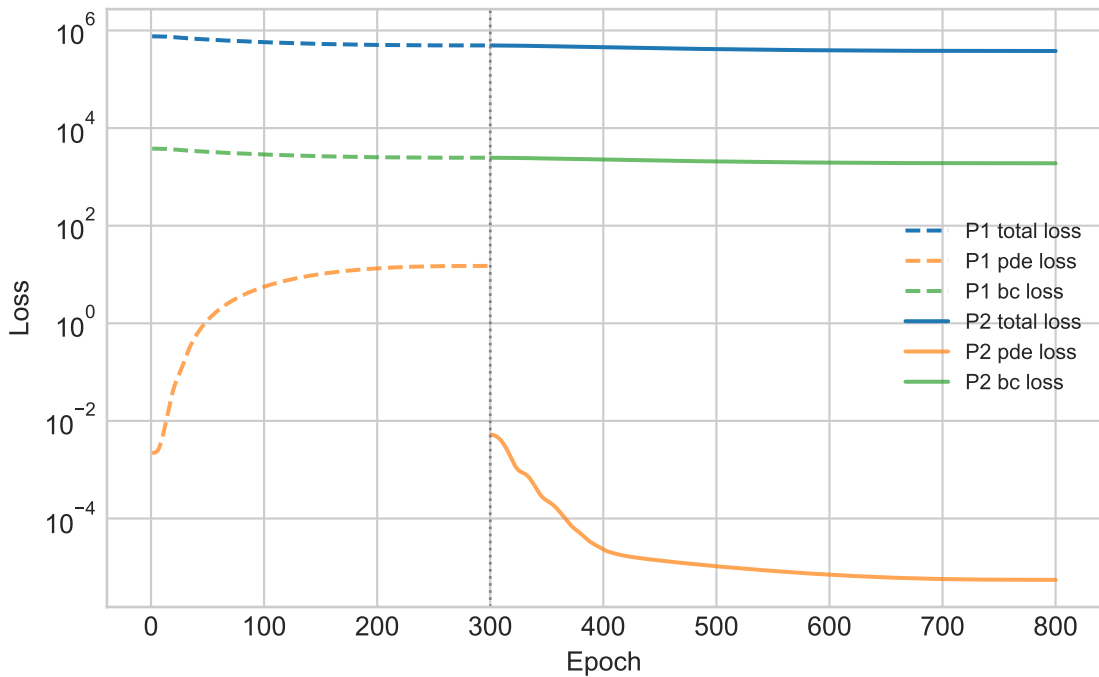
2-site chain: P1 \rightarrow P2A random
