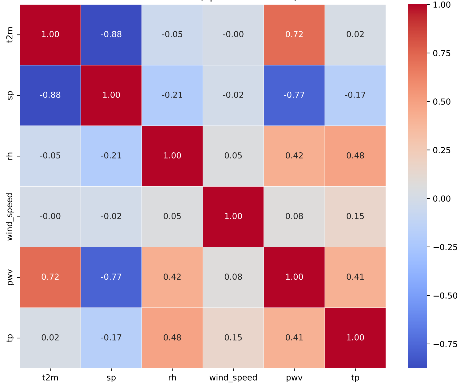
Correlation Matrix (Spearman Method)
