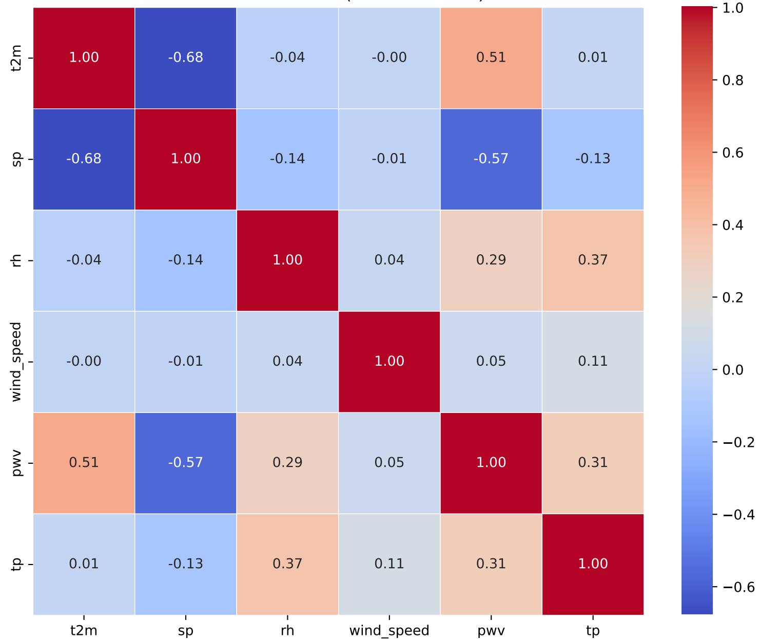
Correlation Matrix (Kendall Method)
