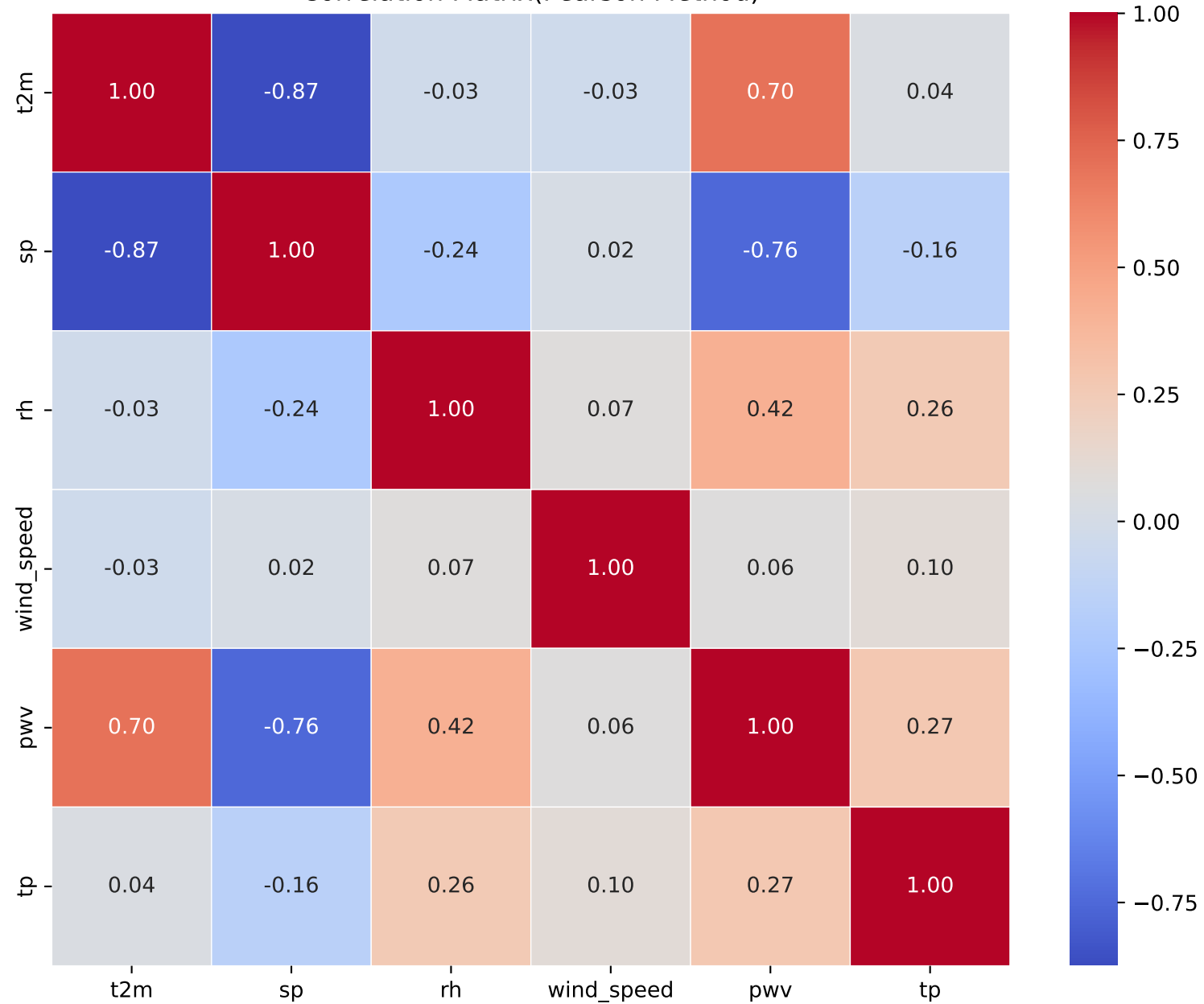
Correlation Matrix(Pearson Method)
