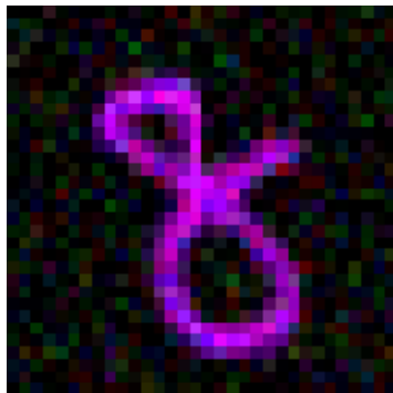
Huber ( \sigma=0.2 )
