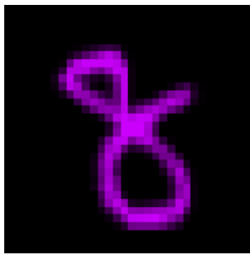
Original (Huber 0)
