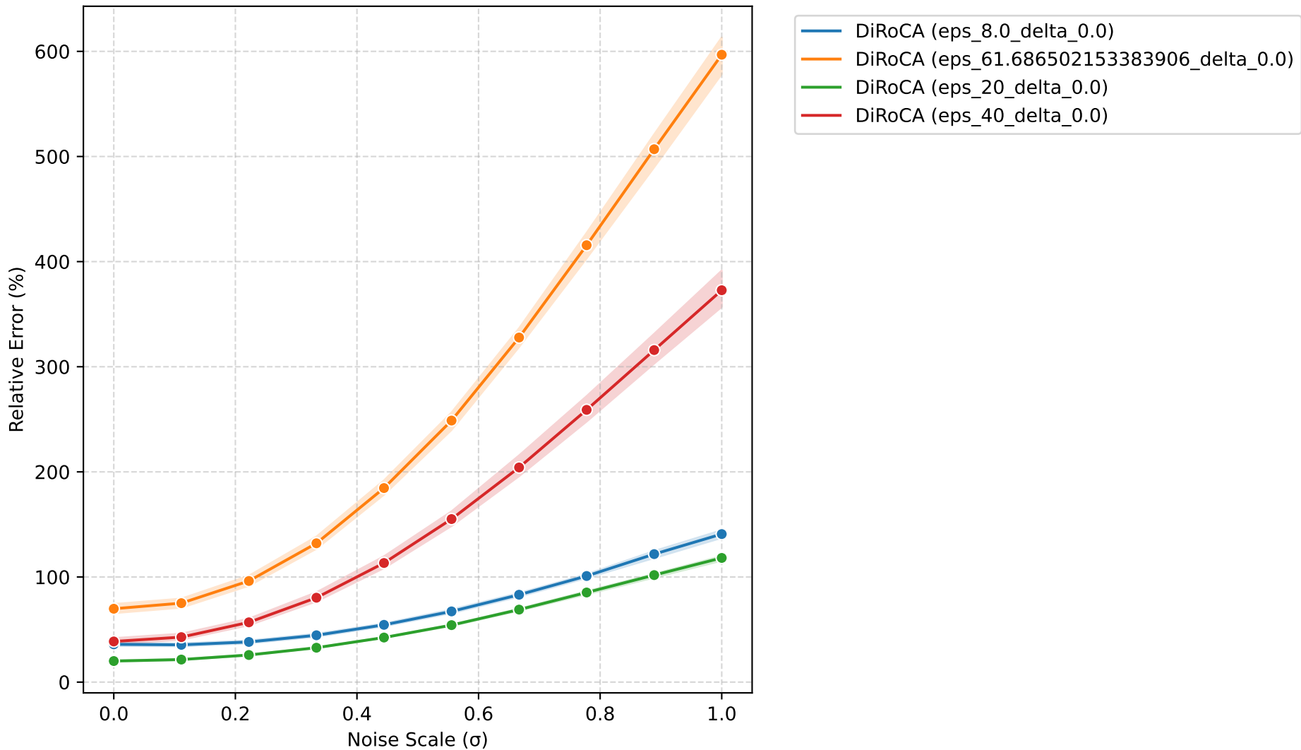
DiRoCA Robustness: Error vs Noise Scale ( \alpha=1.0 )
