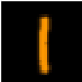
Huber
