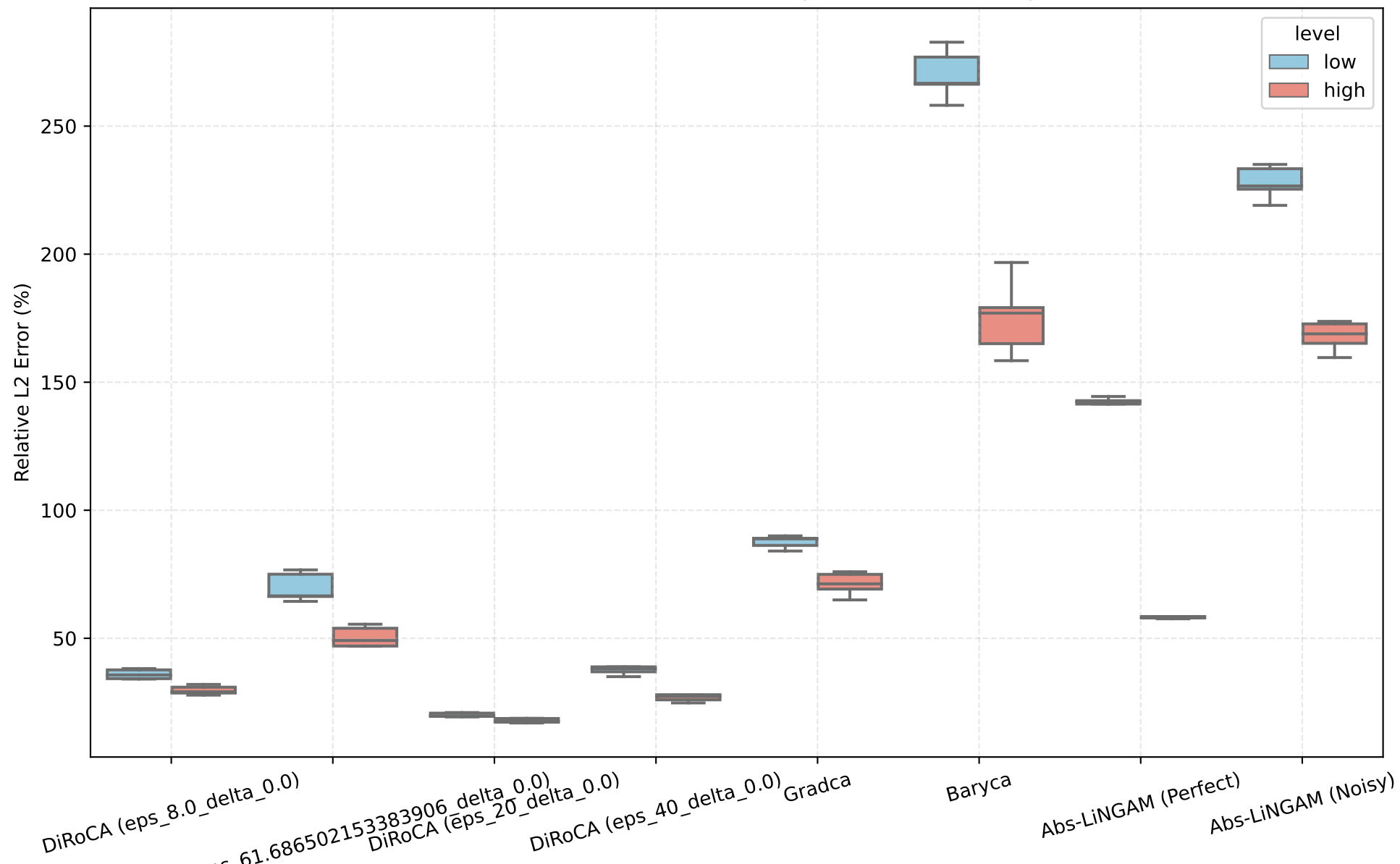
Distribution of Relative L2 Error (Affine Corrected): Blur
