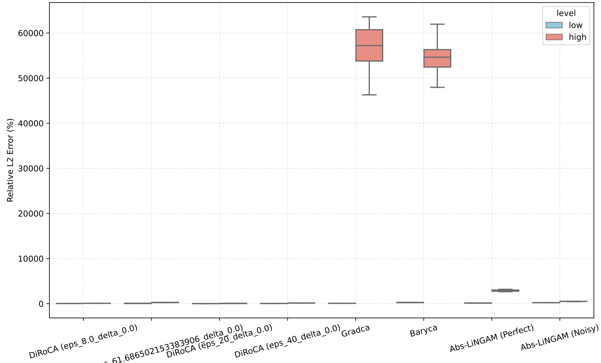
Distribution of Relative L2 Error (Affine Corrected): Angle
