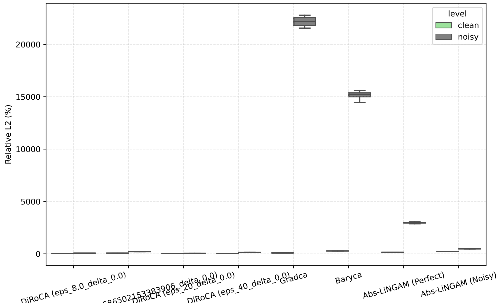
Huber Contamination (Affine Corrected)
