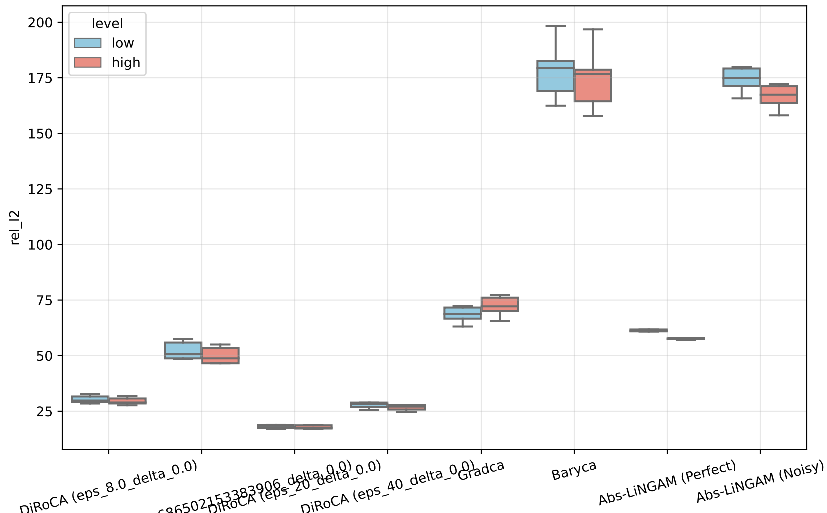
Relative Error: Blur
